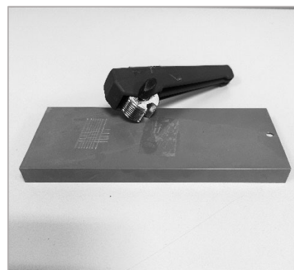
Figure 7 -Cross-cut
